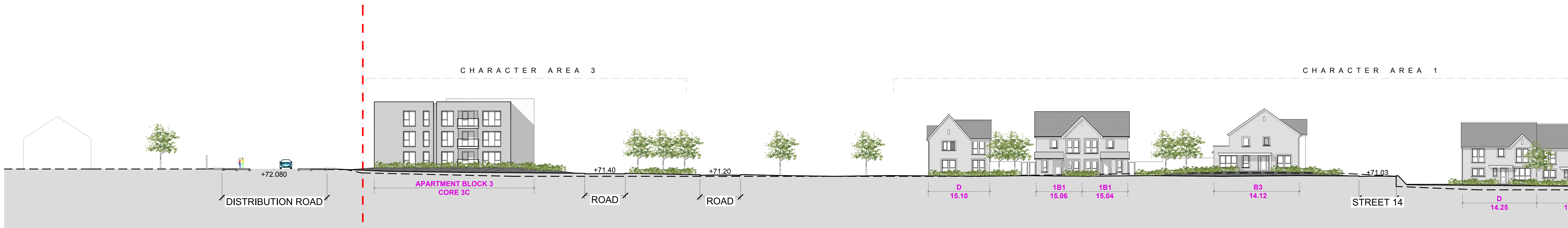
Section BB 1 1:200 @ A0
